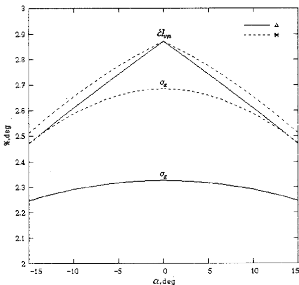
FIG. 3. Methodical error \sigma_\alpha of determination of oblique angle and relative methodical error \delta l_{\text{sys}} of measurement of a linear segment for schemes of triangle and star ( \beta_0 = \beta_0^{\max} ).
