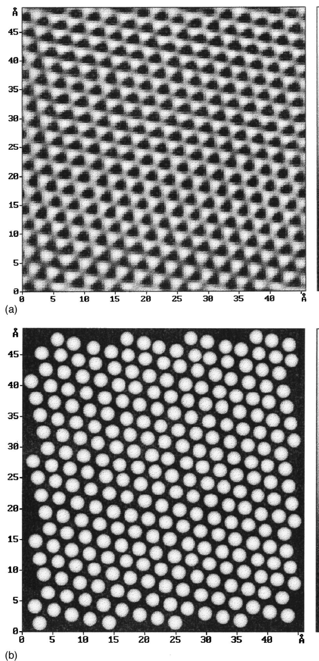
FIG. 1. (a) An example of midsize graphite scan ( 128 \times 128 pixels, microscope is decalibrated). The measurements were made in constant Z mode at U_{\text{tun}} = -100 \text{ mV} , I_{\text{tun}} = 300 \text{ pA} . Average compactness 97.2%. (b) The result of recognition-stylized surface of graphite. Carbon atoms are shown as hemispheres.
